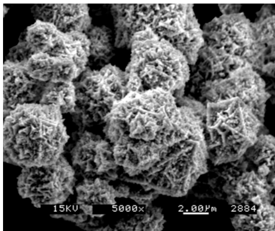
Figure 1 (c) - Morphology of nickel powder observed by SEM.
