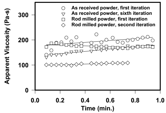
Figure 6 - Apparent viscosity versus time for 60% solid loading feedstock obtained at constant shear rate ( 294.53 s^{-1} ) at Readco continuous mixer.
