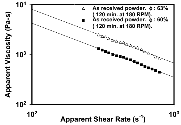
Figure 3 - Variation in the apparent viscosity with shear rate for feedstock of 60 and 63% solids loading. The mixing experiments were conducted in torque rheometer at 180 RPM during 120 min.
